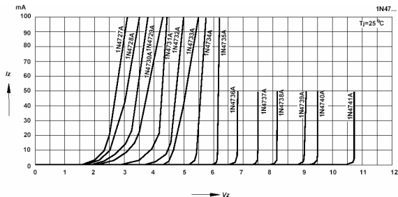
Breakdown characteristics T_J = \text{constant} (pulsed)
